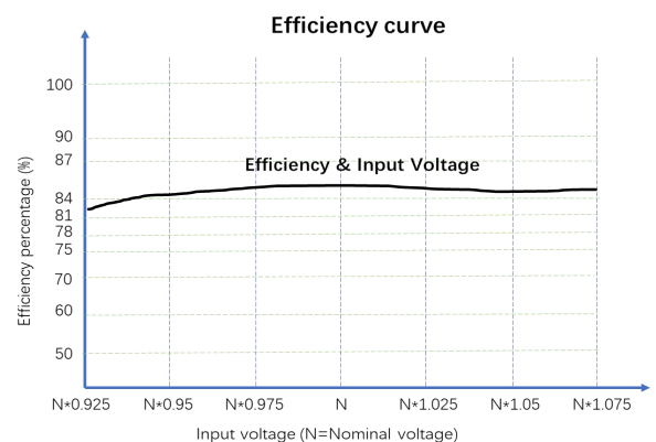
Figure 6: Efficiency VS Input Voltage (100% Load)
