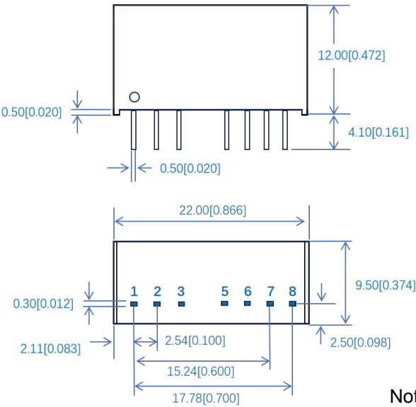
Figure 7: Overall dimensions
