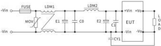
Figure 2: EMC Typical Recommended Circuits 图2:EMC典型推荐电路
