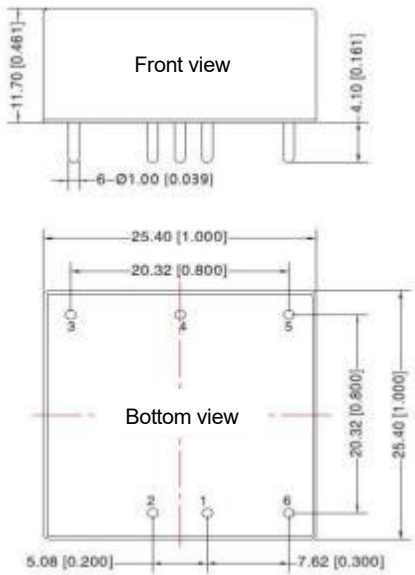
Figure 7: Overall dimensions
