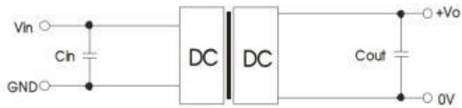
Figure 1: Application circuit
