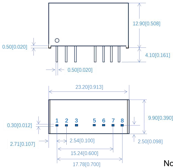
Figure 7: Overall dimensions
