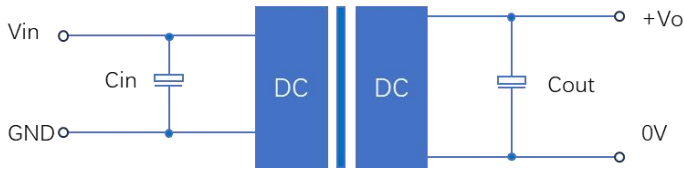
Figure 1: Application circuit
