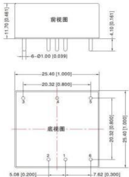
Figure 7: Overall dimensions
