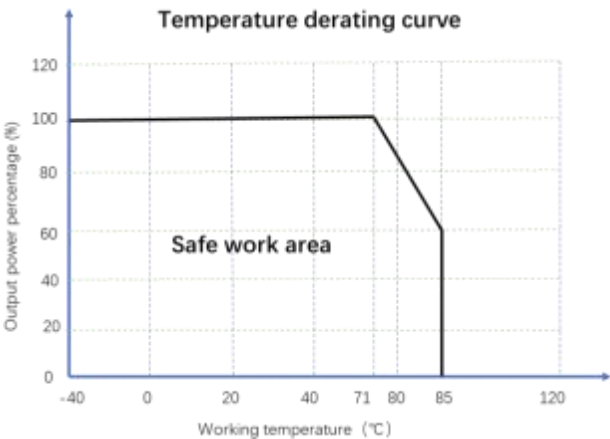
Figure 4: Temperature Derating Curve 图4：温度降额曲线
