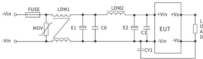
Figure 2: EMC Typical Recommended Circuits 图2:EMC典型推荐电路
