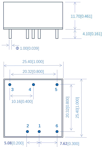
Figure 7: Overall dimensions
