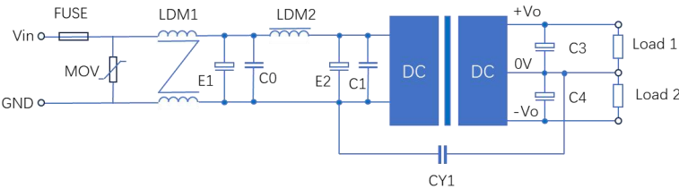
Figure 3: Ripple application and testing 图3:纹波应用及测试
