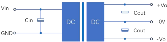
Figure 1: Application circuit 图1：应用电路
