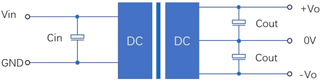
Figure 1: Application circuit 图1：应用电路
