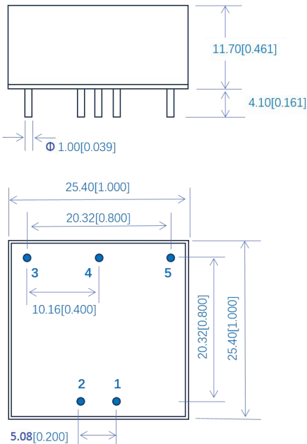
Figure 7: Overall dimensions
