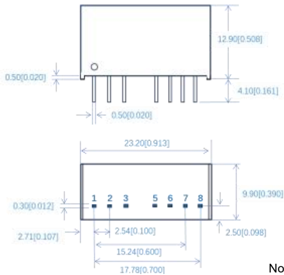
Figure 7: Overall dimensions
