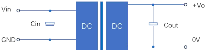
Figure 1: Application circuit 图1：应用电路
